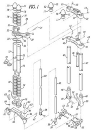
D66 springer Dragon Slayer Patent drawings
